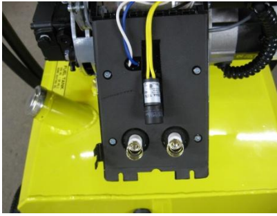
Cad Cell Eye Assembly mounted to the ignitor.
